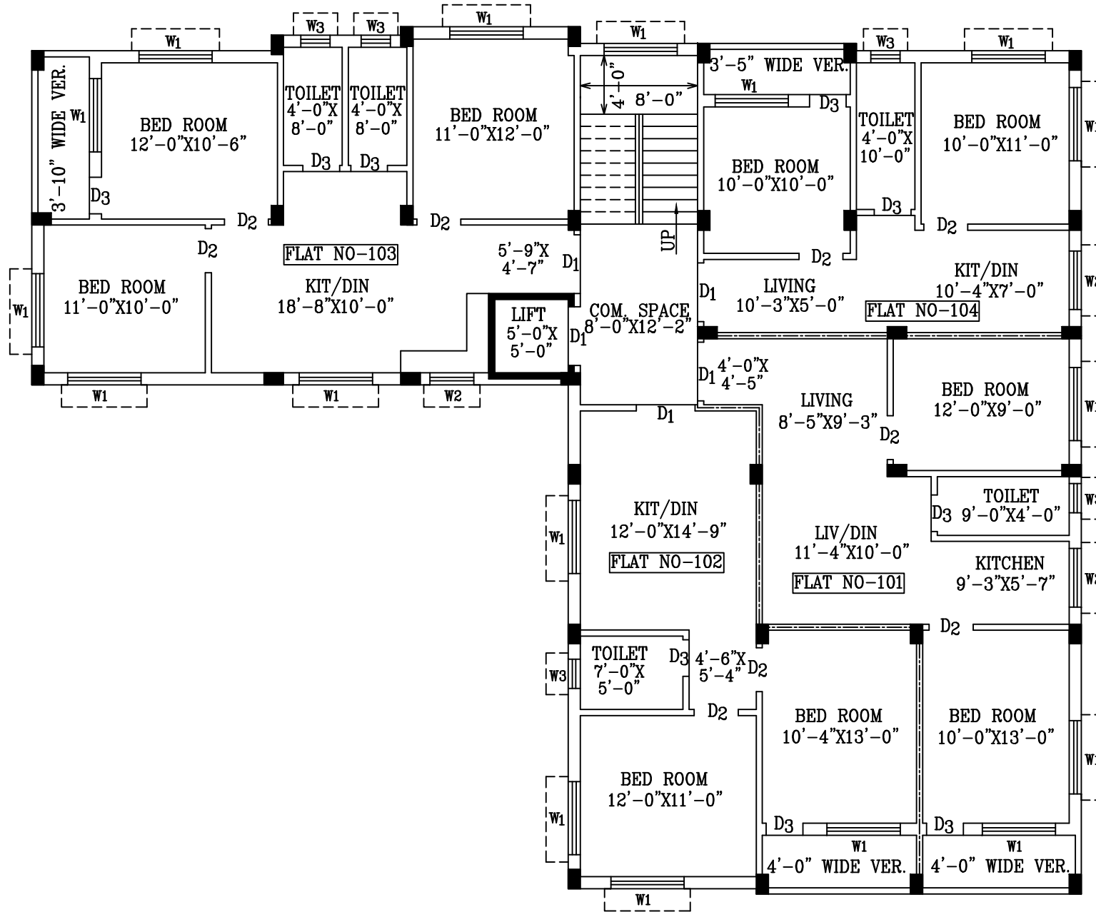
PROPOSED 1ST,2ND,3RD & 4TH FLOOR PLAN
